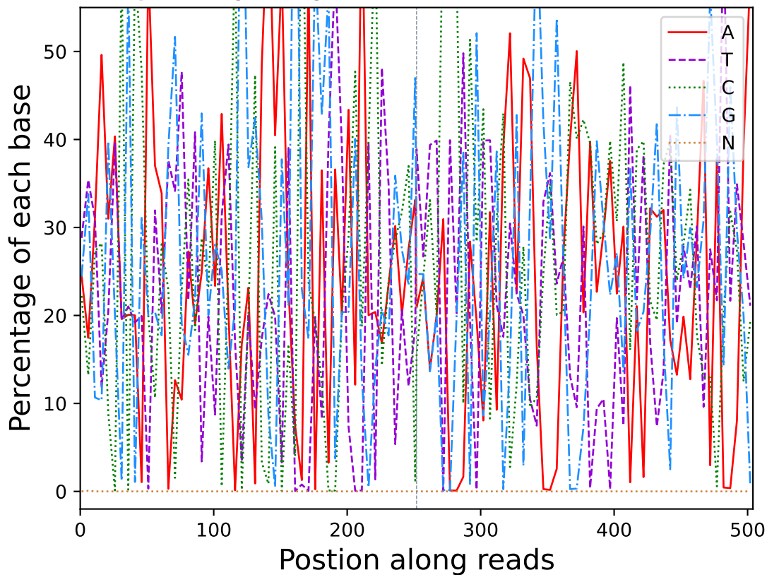
Base percentage along reads (R10910)
